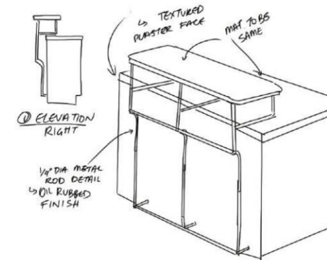
Cantilever Counter Piping Detail
