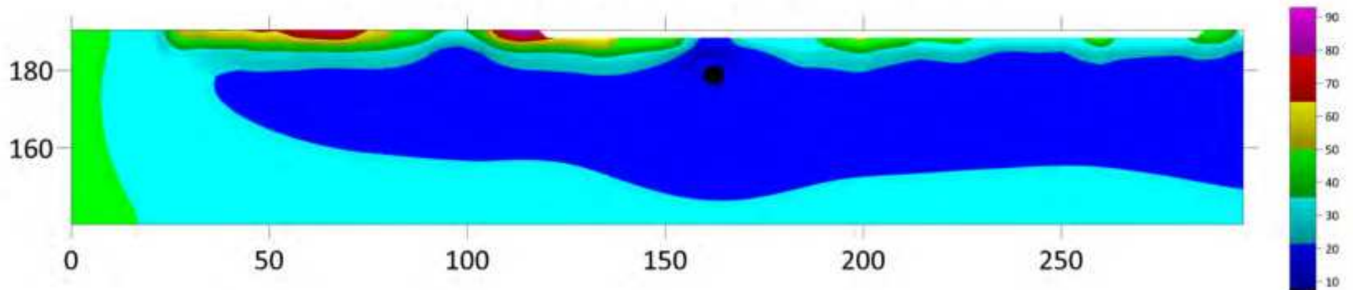
GEOELECTRICAL EAST-WEST LINE 1 - RESISTIVITY
