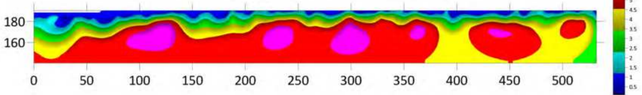
GEOELECTRICAL EAST-WEST LINE 2 - INDUCED POLARIZATION
