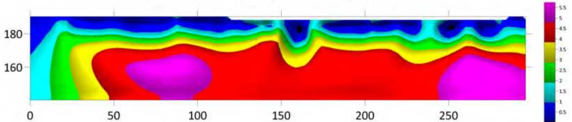
GEOELECTRICAL EAST-WEST LINE 1 - INDUCED POLARIZATION
